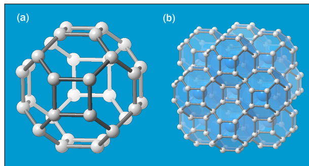
Figure 1: (left) The hydrogenic clathrate cage that is found within Fm\text{-}3m \text{LaH}_{10} and (right) its extended crystal structure.
